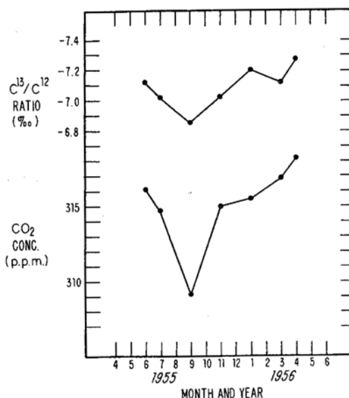
Fig. 4. Variation in concentration and C^{13}/C^{12} ratio of atmospheric carbon dioxide, based on Keeling (1961) for various locations near the Pacific coast of the United States.
