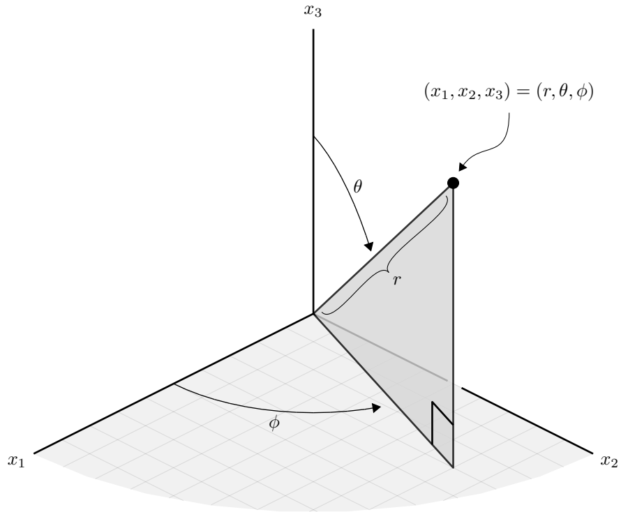
Figure 8.2: Spherical coordinates.
