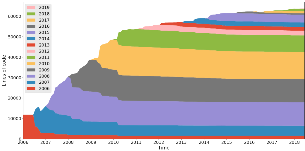
Fig. 3. Clojure codebase—Introduction and retention of code
